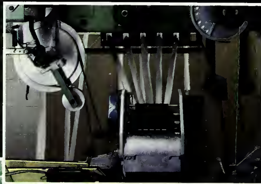
DREF 3 Friction Spinning Machine —Excellent for Core Yarns and Multi-Component Yarns. Count range 3.5c.c. to 18c.c. Delivery speeds to 330 yds/min.
